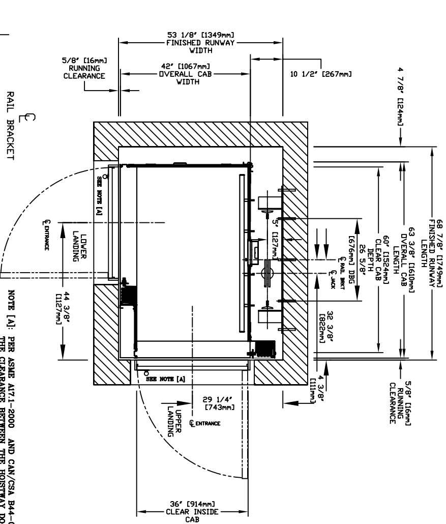
PLAN VIEW - INFINITY Model 3660 TYPE 3
