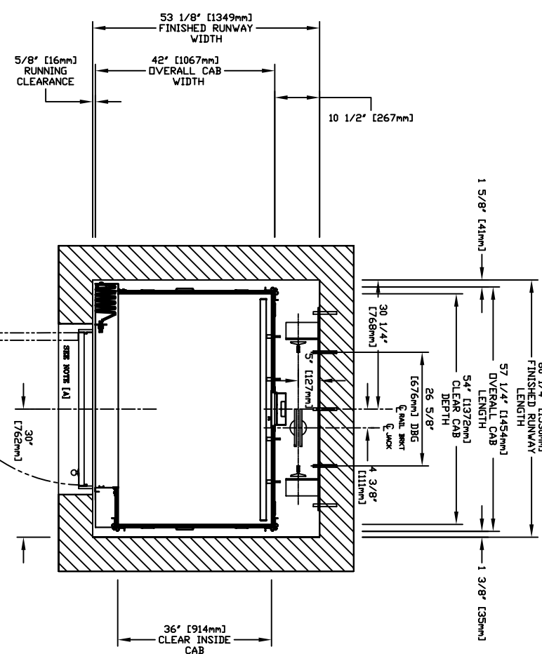
PLAN VIEW - INFINITY Model 3654 TYPE 5
