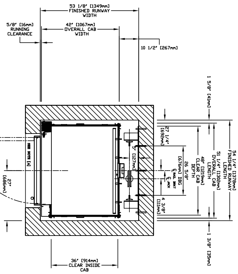
PLAN VIEW - INFINITY Model 3648 TYPE 5
